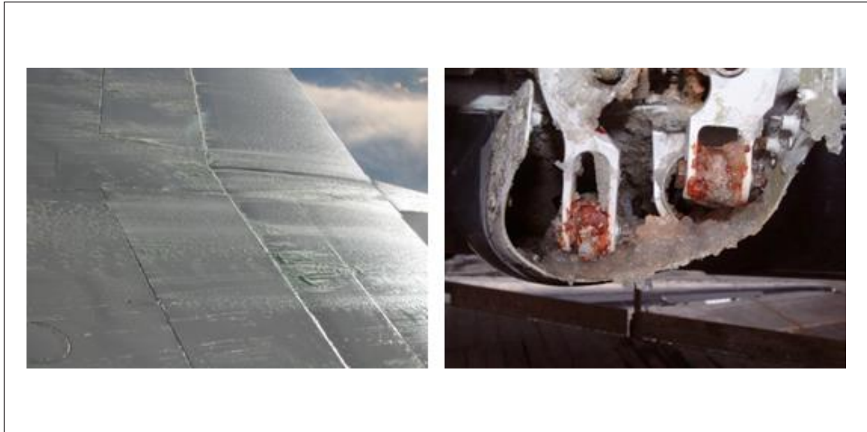
Figure III-9-1. Images showing residual anti-icing fluid frozen on a wing, and fluid dry-out and rehydration on control mechanisms, potentially restricting control movement (Images reproduced by kind permission of NASA.)
