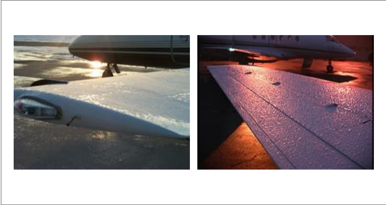
Figure II-1-1. Examples of icing on aeroplane surfaces (Images reproduced by kind permission of NASA.)
