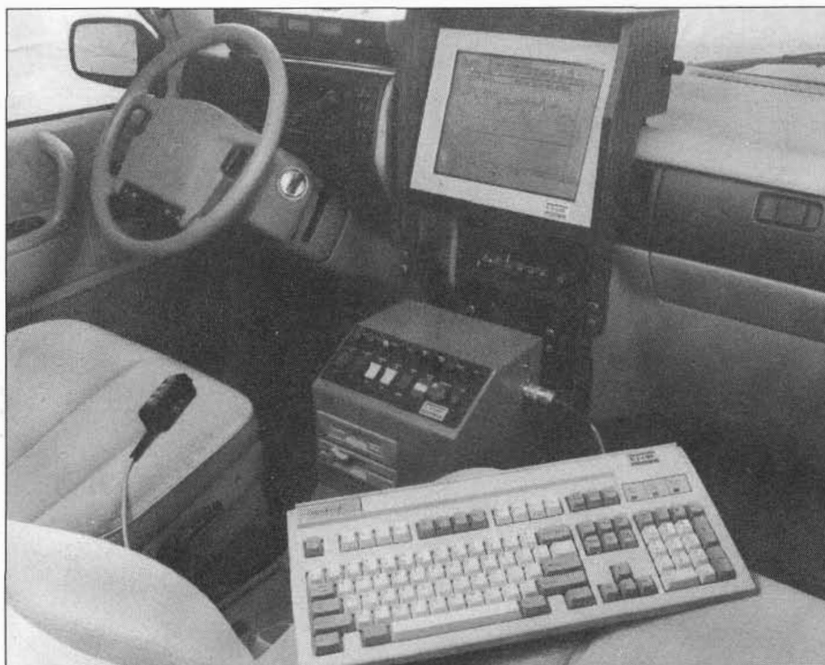
Figure 5-7. The vacuum fluorescent display unit and keyboard for the Runway Friction Tester
