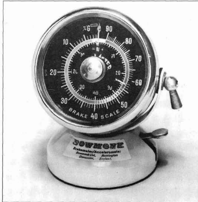
Figure 5-14. Brakemeter-Dynometer
