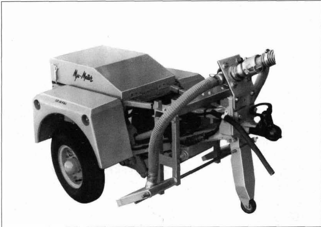
Figure 5-4. Mu-meter trailer
