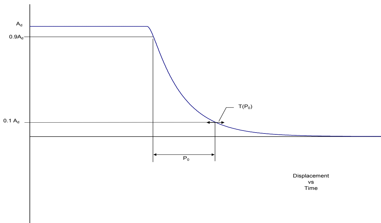
Figure 2 : Critically damped step response
