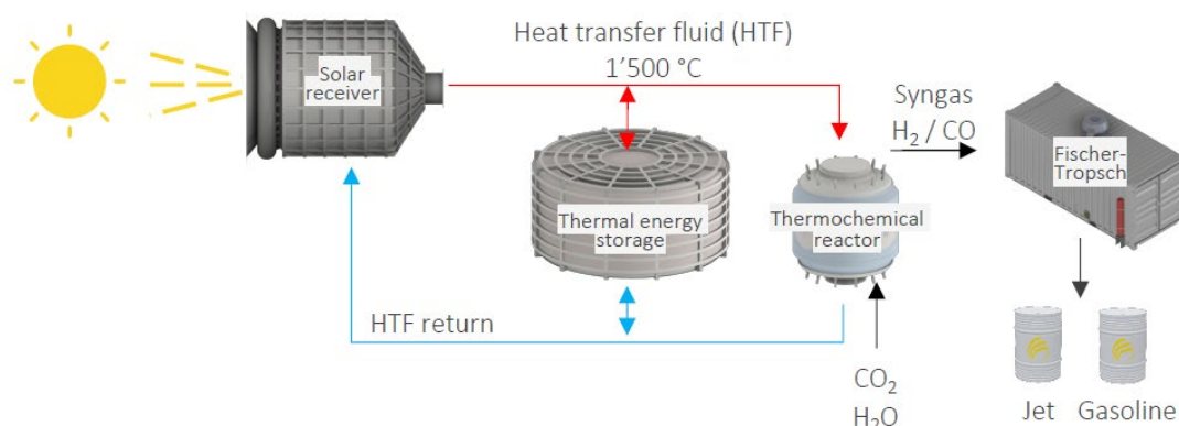
Flow scheme 5: Design of a Synhelion pure thermochemical syncrude production pathway. \text{CO}_2 and \text{H}_2\text{O} are split in a ceria-based redox process to produce syngas. The syngas of all towers is centralized and processed to syncrude at one single location in conventional Fischer-Tropsch synthesis plant. The solar field not shown includes the heliostats for the reforming. Figure: Courtesy of Synhelion.
