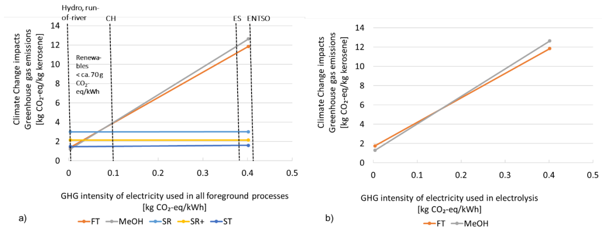
Figure 12: Performance in climate change impacts of the production of 1 kg synthetic kerosene via various PtL or StL pathways in relation to the input electricity used a) in foreground processes, namely CO 2 capture, H 2 production, and processing, or b) in electrolysis (thus only shown for PtL). CH = Switzerland, ES = Spain, ENTSO = European electricity mix
