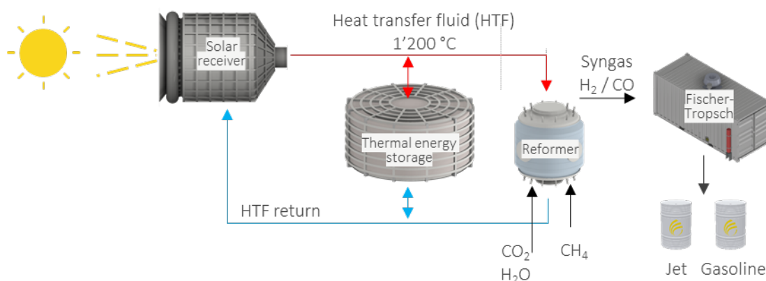
Flow scheme 3: Design of a Synhelion solar reforming syncrude production pathway. High-temperature solar reforming of CH 4 takes place together with its reaction with CO 2 and H 2 O to produce syngas. The syngas of all towers is centralized and processed to syncrude at one single location in conventional Fischer-Tropsch synthesis plant. The solar field not shown includes the heliostats. Figure: Courtesy of Synhelion.
