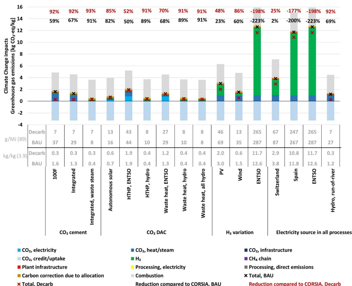
Figure 15: Contribution analysis of climate change impacts of the Methanol PtL pathway with various variations of input parameters to explore potential optimisation possibilities.
