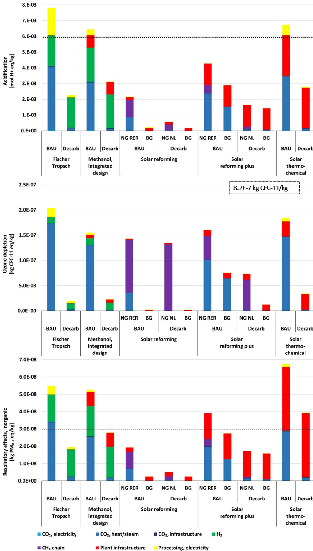
Figure 13 Results for selected life cycle impact assessment categories for the production of 1 kg synthetic kerosene. The dotted line (or the value in the dotted box, respectively) shows the score for conventional kerosene.
