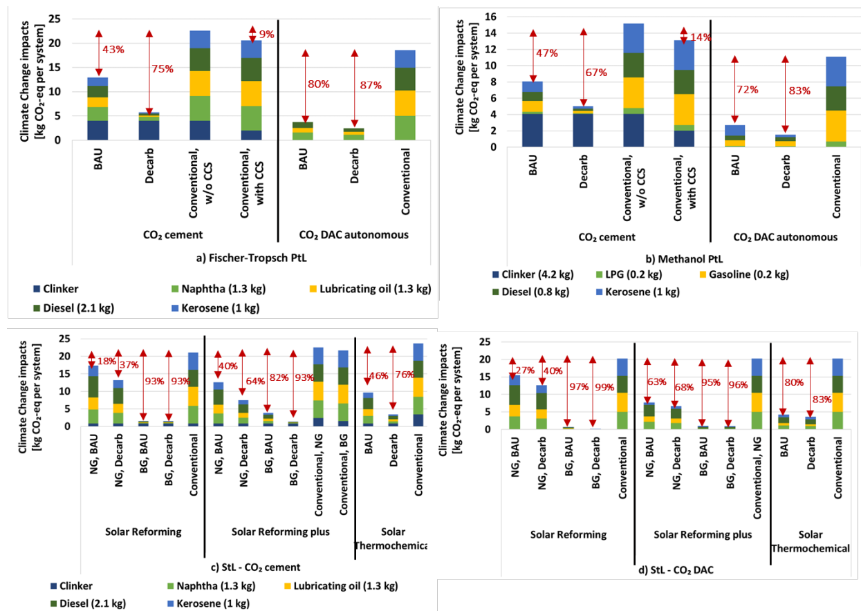
Figure 20: System perspective on climate change impacts of fulfilling a demand in fuels with conventional production pathways or via PtL (top, (a) and (b)) or StL (bottom, (c) and (d)). The PtL figures are again split into two parts: One for a system where the CO 2 comes from the cement plant, and one where it is captured from air (thus no clinker involved). The reduction potential is shown with red arrows.
