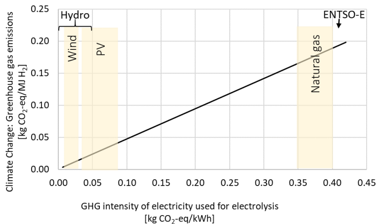
Figure 10: Climate change impacts of the production of 1 MJ hydrogen via water electrolysis in a PEM electrolyser as a function of the greenhouse gas intensity of the input electricity. No storage is considered for the pure renewable cases. Taken from own publication (Antonini et al. 2020).
