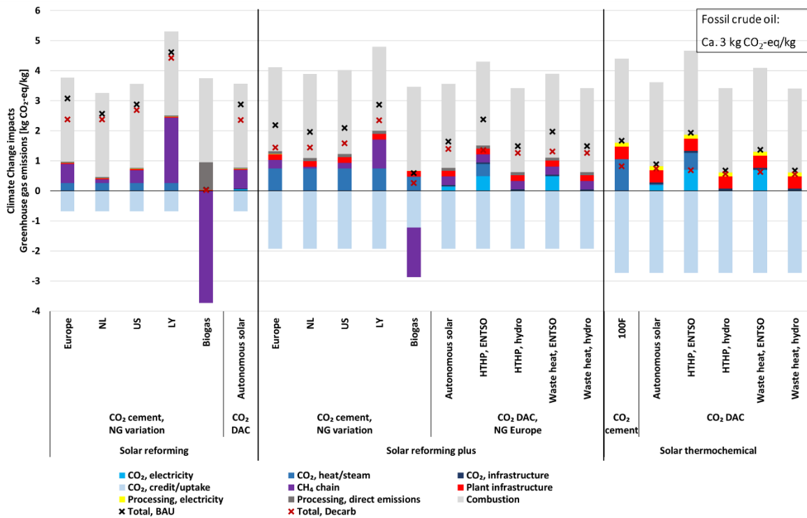
Figure 16: Contribution analysis for climate change impacts of the production of 1 kg syncrude via the StL pathways. Bars show contributions to total BAU scores. Refining to useable fuels is not included.
