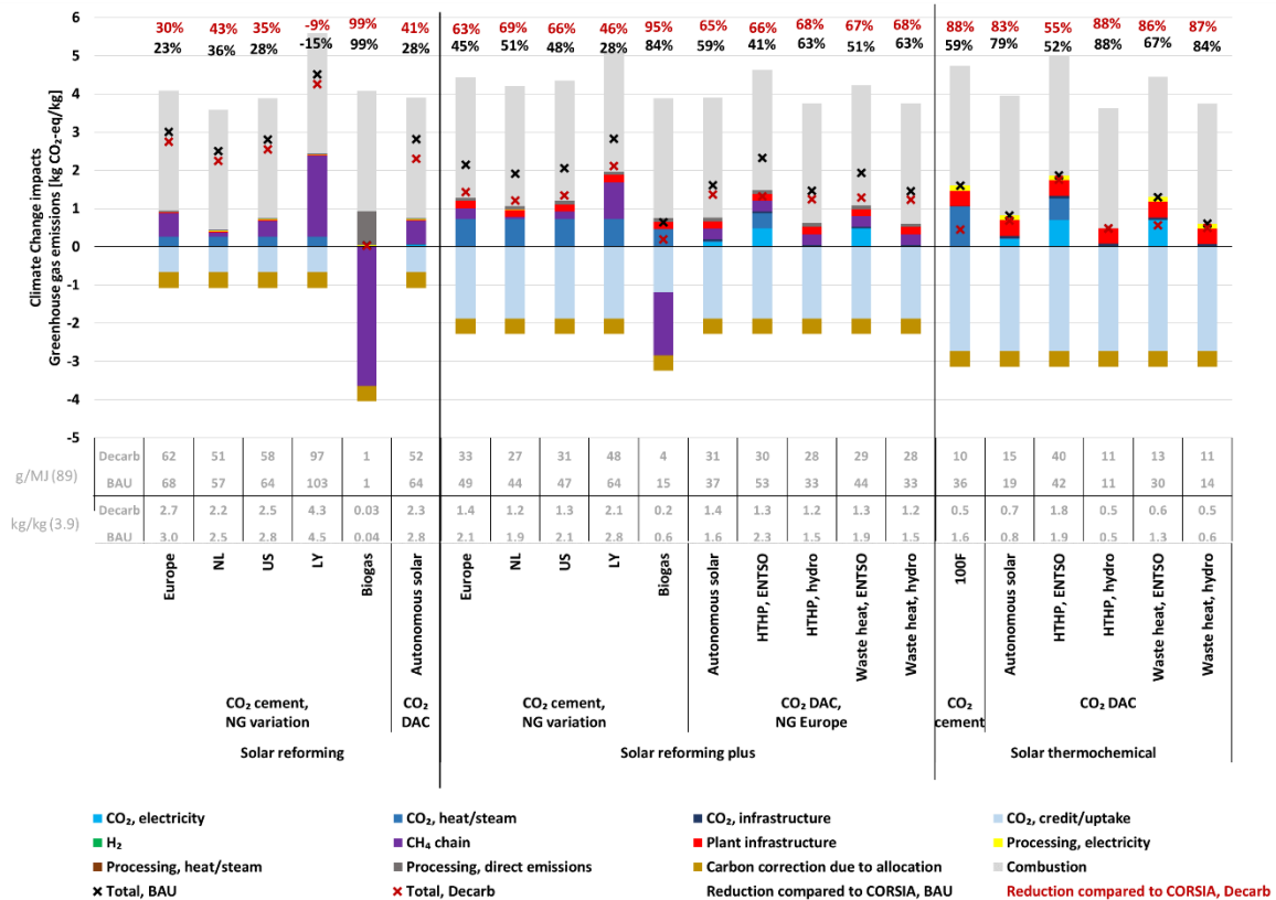
Figure 17: Contribution analysis of climate change impacts of the Synhelion StL configurations with various variations of input parameters to explore potential optimisation possibilities. Results are shown for all three configurations, with variation of the natural gas source, DAC design, and integrated pure solar cement plant.
