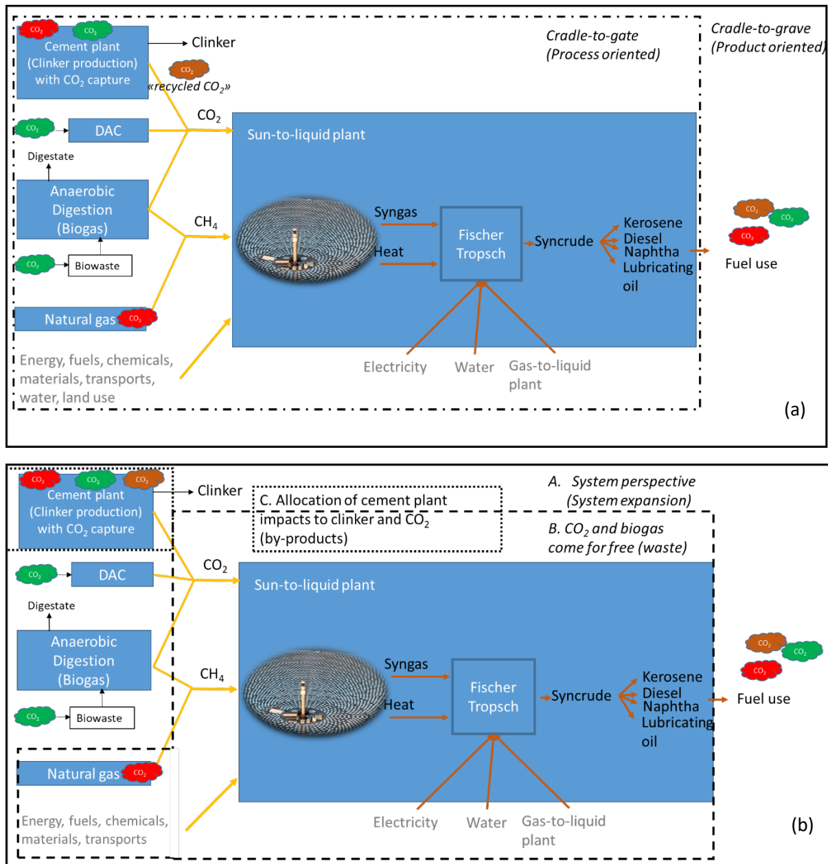
Figure 3 System boundaries chosen to model synthetic fuel production via the Sun-to-Liquid pathway. The upper figure (a) shows the two perspectives of the fuel producer (cradle-to-gate, oriented for optimizing the producing process) on the one hand, and the fuel user perspective on the other hand (cradle-to-grave, oriented to comparing a product with others fulfilling the same need). The figure at the bottom (b) shows a zoom on the various approaches which can be adopted to solve multi-functionality. Grey processes represent background processes, which are taken from databases or previous work by the authors. Processes within the blue boxes are foreground processes. Red CO 2 emissions stand for fossil CO 2 , while the green clouds represent biogenic carbon. "Recycled" CO 2 from CCU is represented with a brown cloud.
