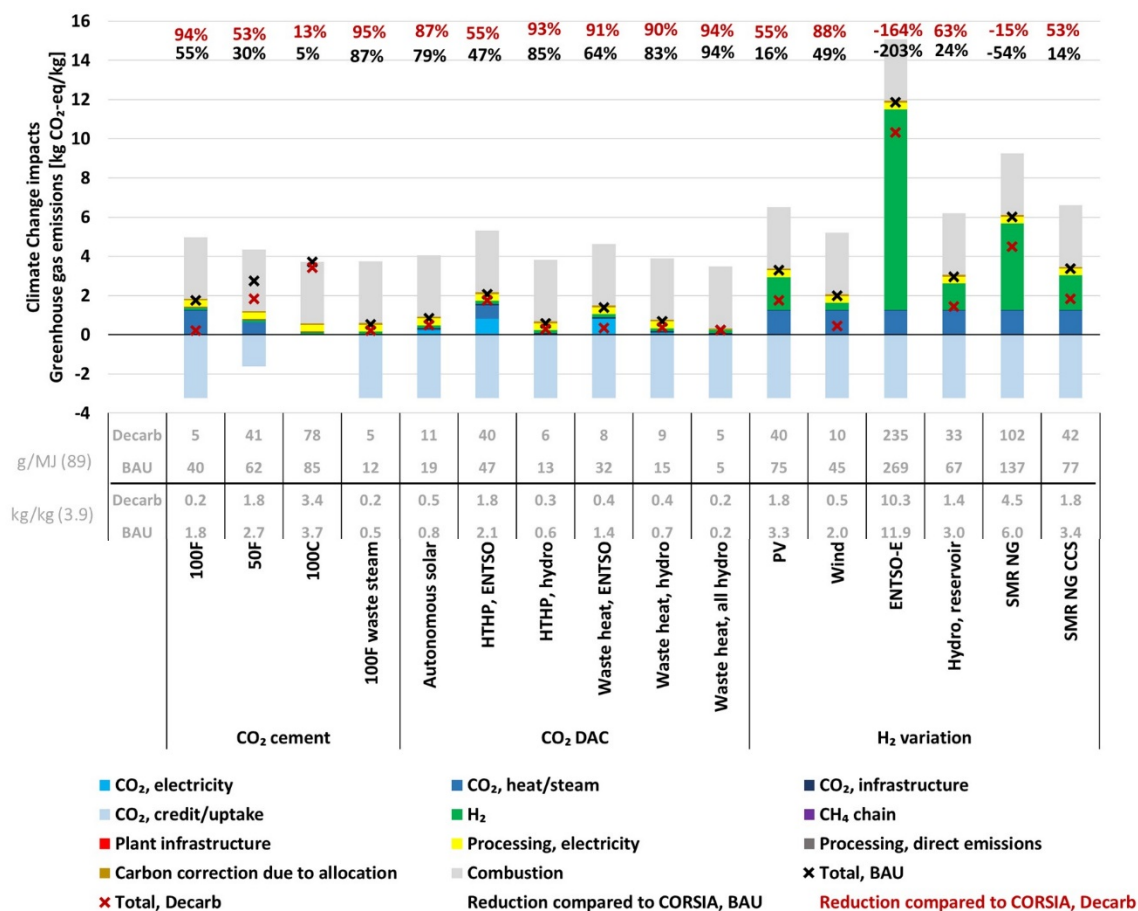
Figure 14: Contribution analysis of climate change impacts of the Fischer-Tropsch PtL pathway with various variations of input parameters to explore potential optimisation possibilities.
