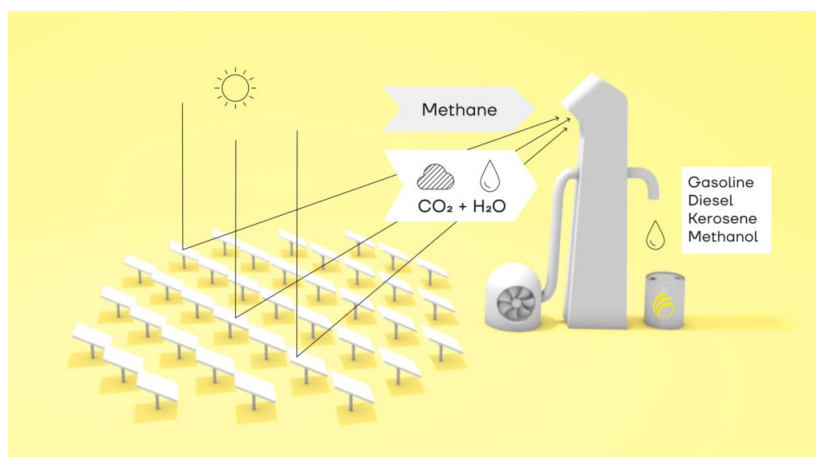
Figure 7: Production scheme of the Synhelion plant.
