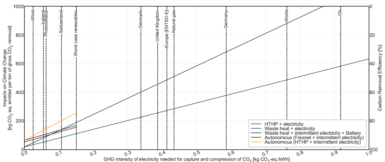
Figure 8: Impacts on climate change per ton CO 2 removed from the air with various DAC plant configurations shown as a function of the greenhouse gas intensity of the input electricity for capture and compression of CO 2 . Taken from (Terlouw et al. 2021). HTHP + electricity = Heat from High-temperature heat pump with electricity as input to the HTHP and to electricity needs.
