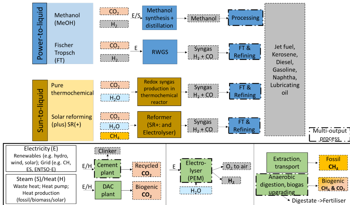
Figure 1: Simplified PtL and StL pathways, with underlying inputs shown in the box at the bottom. The slash-dotted boxes indicate multi-output processes where choices have to be made on how to attribute environmental burdens of the process to the individual co-products. RWGS = reverse water gas shift; DAC = direct air capture; FT = Fischer Tropsch. Within FT, the syngas is converted into liquid hydrocarbons, which are then refined to the desired fuels.
