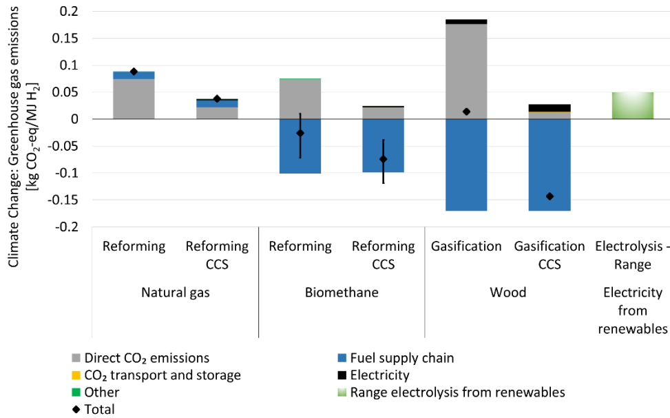
Figure 9: Climate change impacts of production of 1 MJ hydrogen via reforming of natural gas or biomethane with or without CCS as well as the gasification of wood. The black error bar in the biomethane cases represent the variability in the carbon balance from biomass (with highly varying C content and fate of C in the digestate co-product of biogas) up to hydrogen. The potential range of climate change impacts from electrolysis depending on the input electricity is shown for comparison on the right side. Based on (Antonini et al. 2020, 2021).
