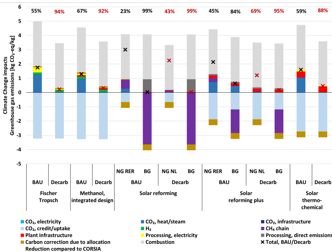
Figure 11: Contribution analysis of climate change impacts of the production of 1 kg kerosene via various PtL and StL pathways with CO 2 from cement plant. Combustion of the kerosene in an aircraft engine is considered only via emission of CO 2 to air associated with carbon embodied in the kerosene; no other climate effects of aircraft are considered. The red figures indicates the reduction of greenhouse gas emissions compared to the CORSIA benchmark. BAU = Business-as-usual scenario; Decarb = Decarbonisation scenario. NG = Natural gas, BG = Biogas, RER = Europe, NL = The Netherlands. Conventional kerosene comes with 3.9 kg CO 2 -eq/kg.
