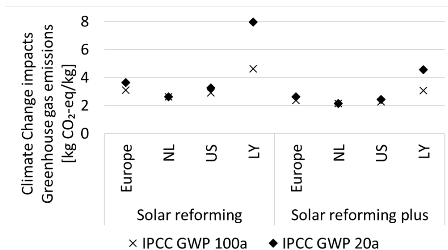
Figure 19 Climate change impacts of synthetic kerosene produced via solar reforming of natural gas with varying origin, calculated with a time horizon of 100 years and of 20 years, respectively, as suggested by the IPCC.
