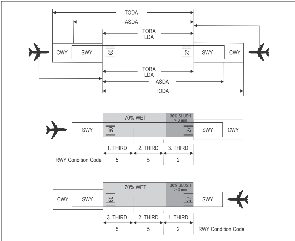
Figure II-2-1. Reporting of runway condition code from ATIS to flight crew for runway thirds
